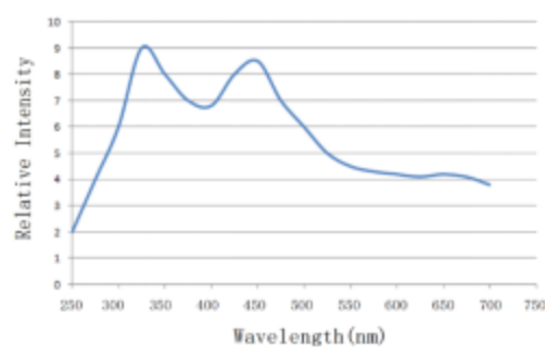
Fig2. Visible light spectrum response curve
