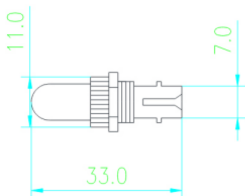
Probe head
