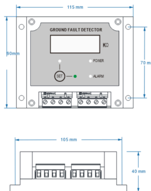
ZJJ-4SC: Din-rail Mounting
